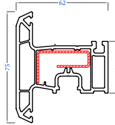
Window Sash - Outward Open PC62-US-01
