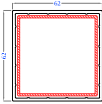
62mm Square Post PA62-UO-01
