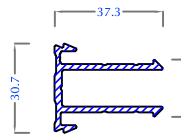
Hurrican Bar 3 Base PAM 127
