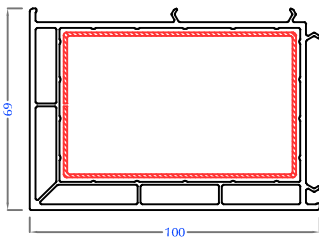
Inventa 2.5 Track Coupler PA62-UO-03
