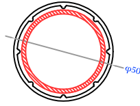
50mm Round Post PA-UO-01
