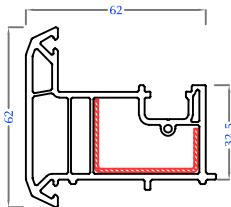
Movable Mullion PC62-UT-03
